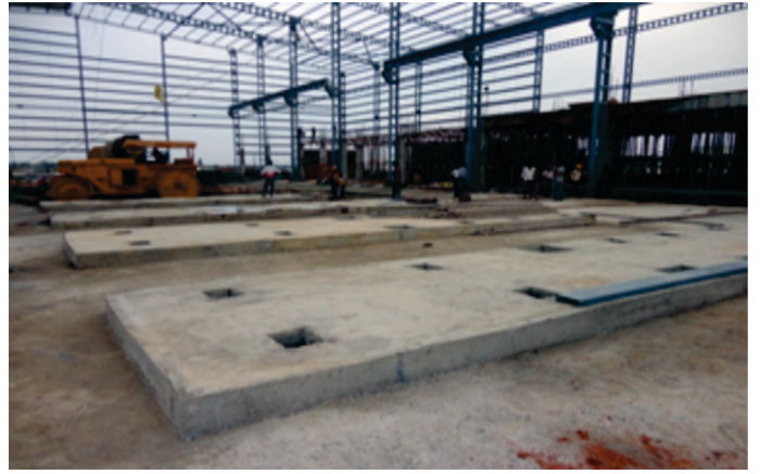
M/S Varroc Polymers Pvt Ltd (Oragadam-Chennai) Machine Foundation
